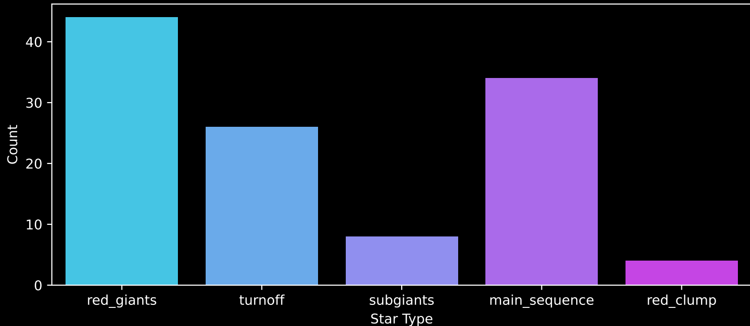
APOGEE DR17 Field: [279-32-O] Count plot of Star Type
