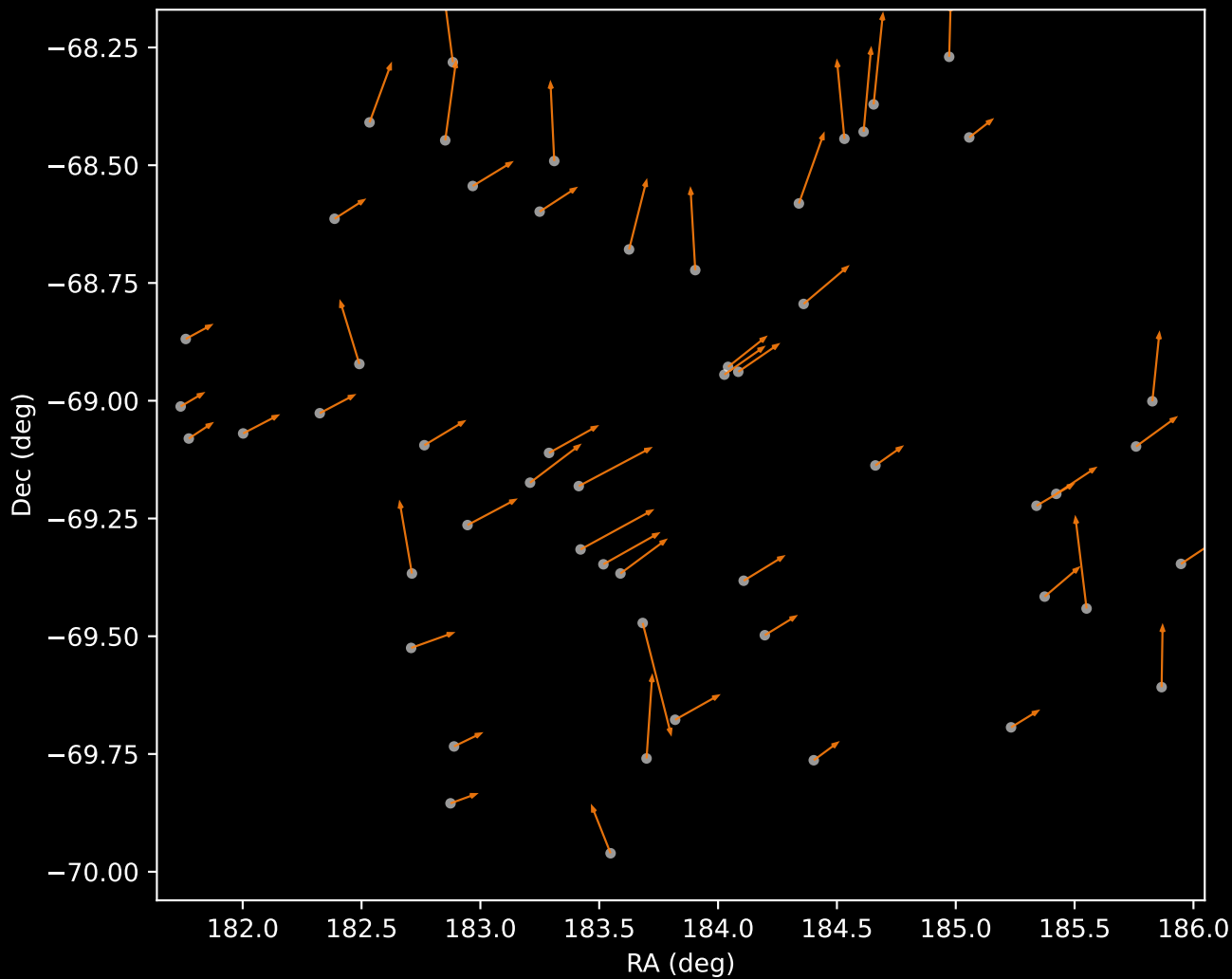
APOGEE DR17 Cluster 2 Proper Motion Vectors (n=54)
