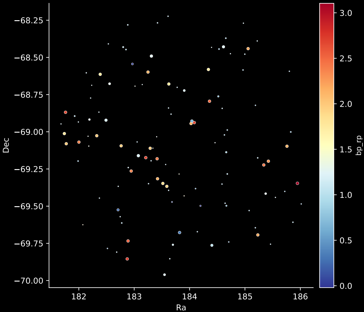
APOGEE DR17 Field: [279-32-O] Stars: 116
