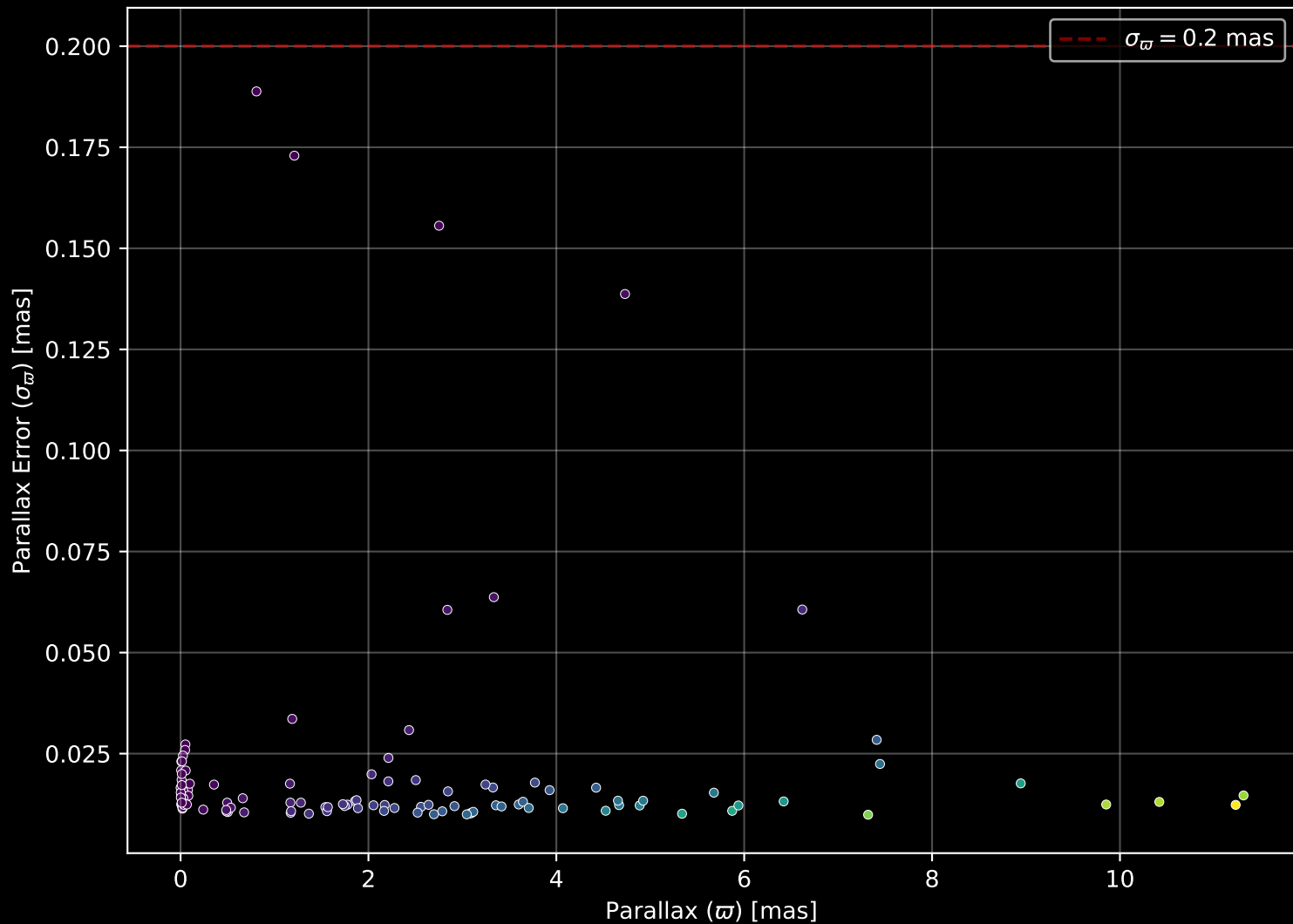
APOGEE DR17 Field: [279-32-O] Parallax Quality (n= 116)
