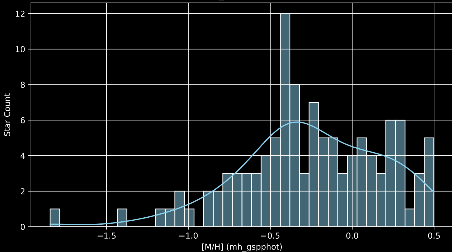
APOGEE DR17 Field: [279-32-O [M/H] (mh_gspphot) (n= 112)
