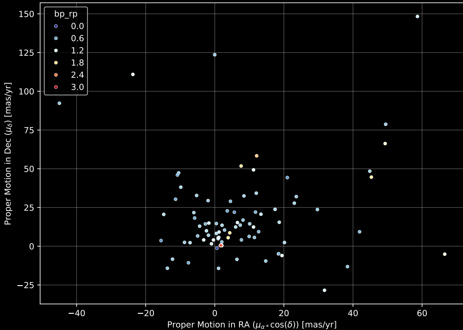
APOGEE DR17 Field: [279-32-O] Proper Motion Diagram (n= 116)
