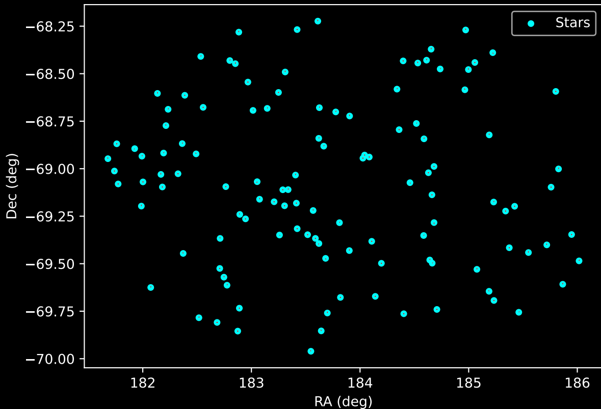
APOGEE DR17 Field: [279-32-O] Proper Motion Vectors for Gaia Star Field (n= 116)
