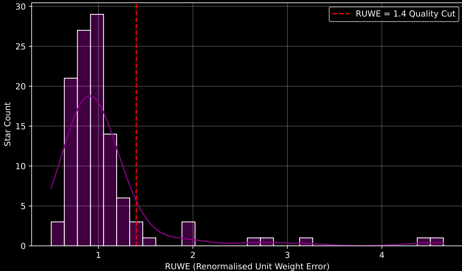
GAPOGEE DR17 Field [279-32-O] RUWE Distribution (n= 112)
